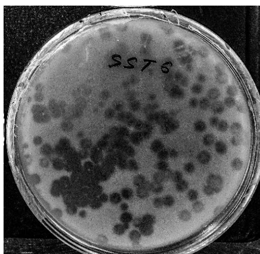
Fig. 1: E. coli MDR strain susceptible to phage ASEC2202
