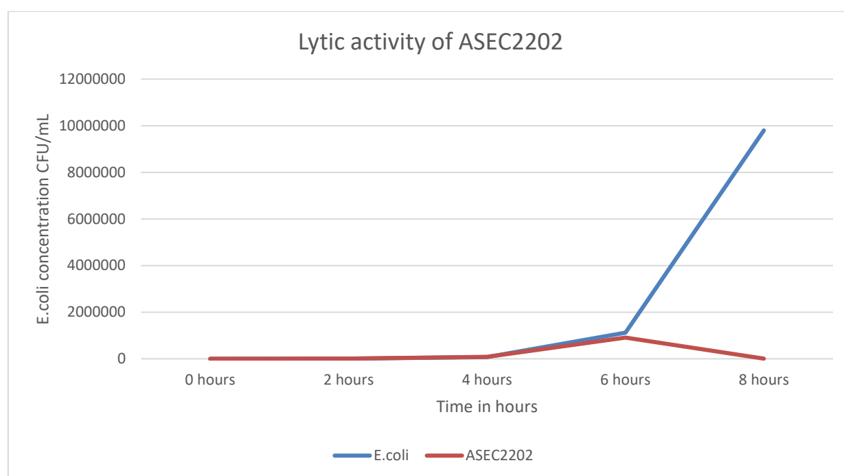
Fig. 3: Lytic activity of ASEC2202 against MDR strain of E. coli at 37 °C at different intervals. The coliphage effectively reduced the viable bacterial cells within 8 hrs.
